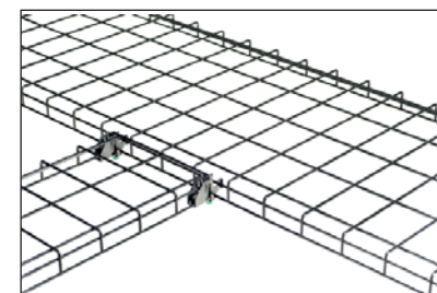
Wyr-Grid™ Pathways No Sidewall Removal Required
